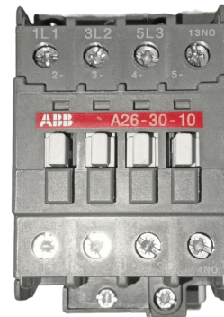
Contactor A26-30-10 110V 50Hz / 110-120V 60Hz 1SBL241001R8410
