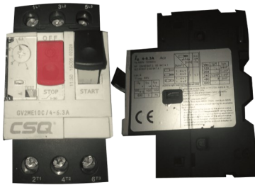
Guardamotor Regulable 4,0-6,3A CSQ GV2ME10C / 4-6.3A
