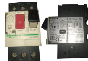
Guardamotor Regulable 13-18A Schneider Electric GV2ME20
