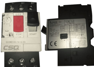
Guardamotor Regulable 4,0-6,3A CSQ GV2ME10C / 4-6.3A
